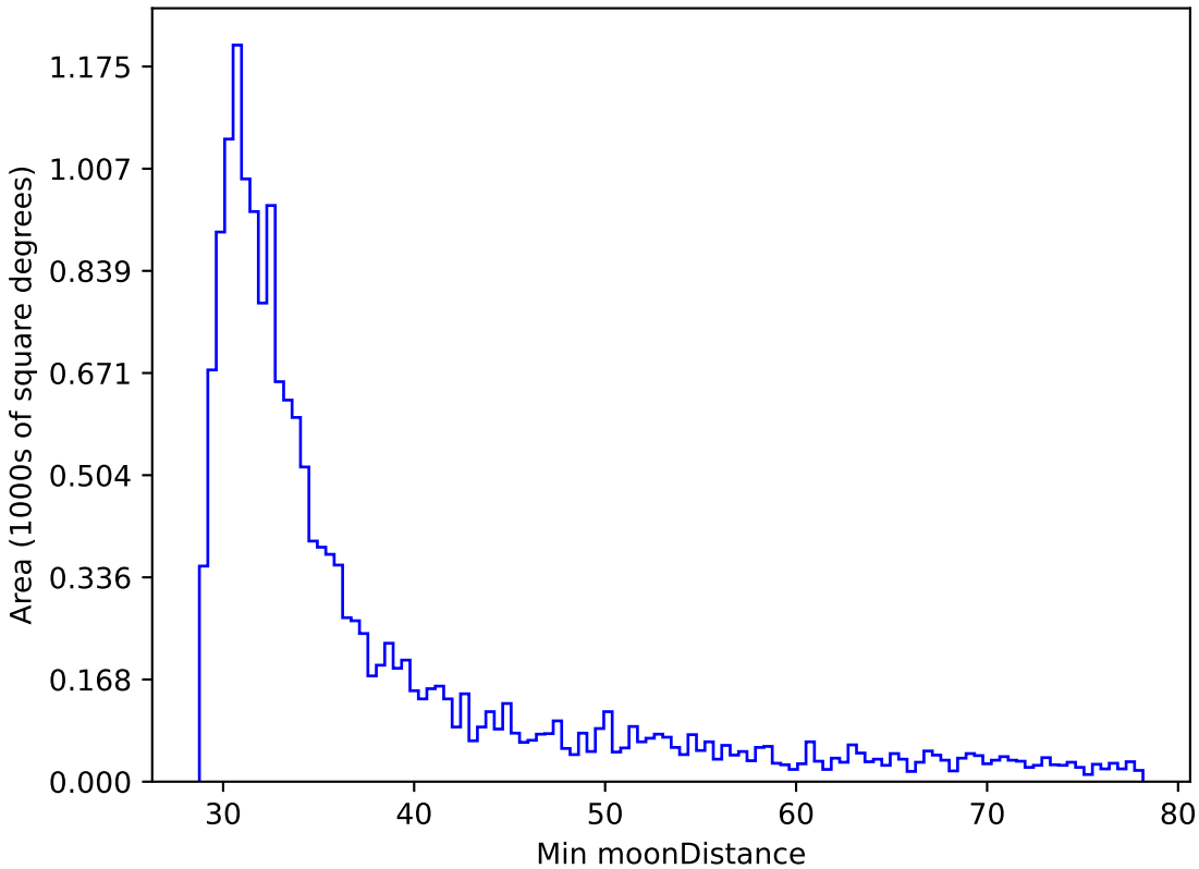
too_ignore_5_1v3.4_10yrs WFD r band: Min moonDistance
