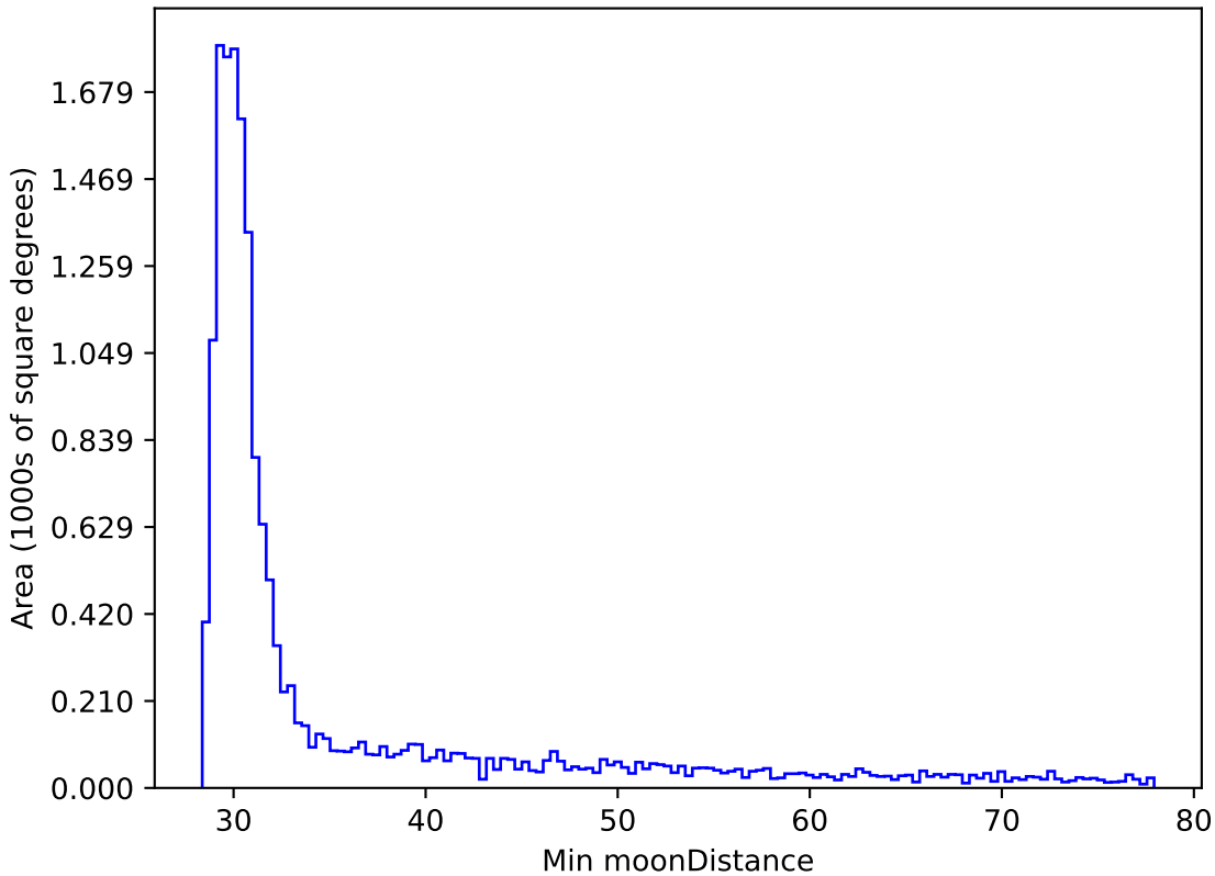
too_ignore_5_1v3.4_10yrs WFD i band: Min moonDistance
