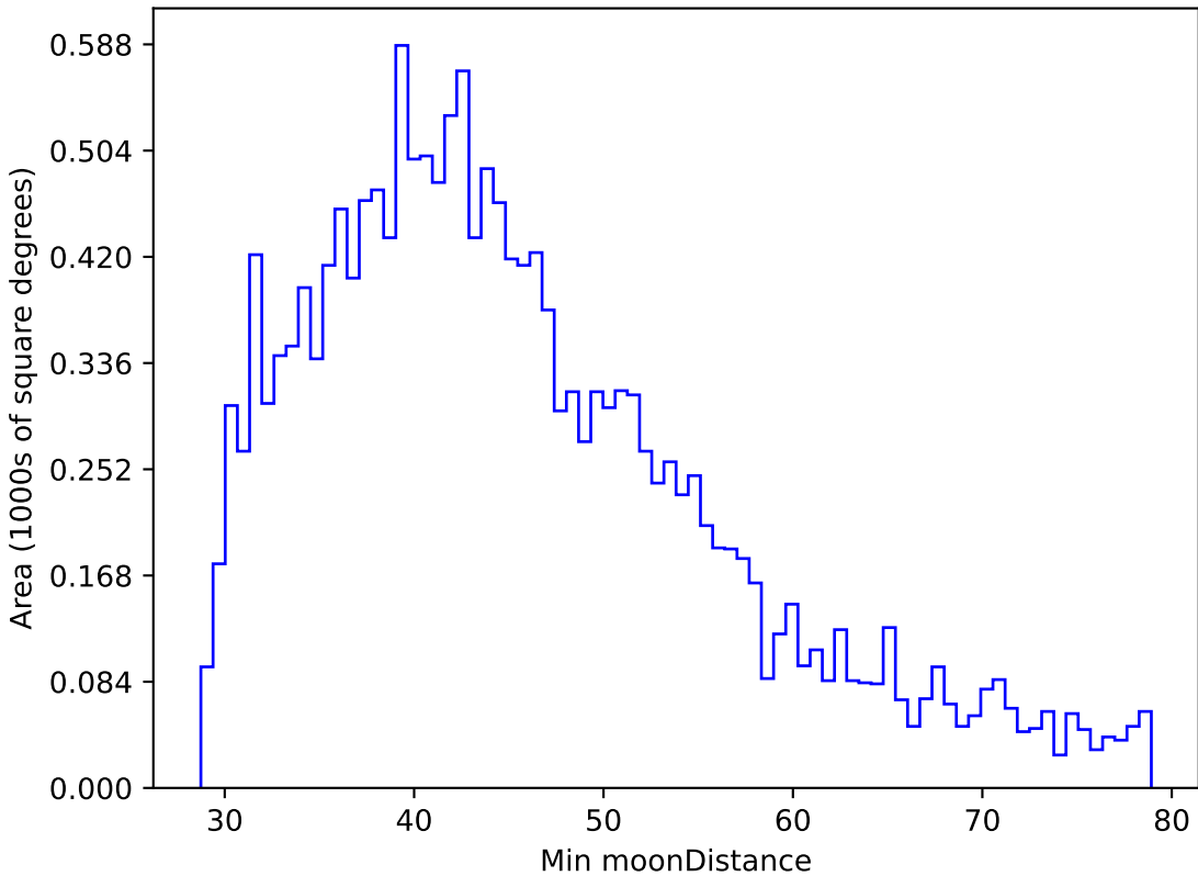
too_ignore_5_1v3.4_10yrs WFD g band: Min moonDistance
