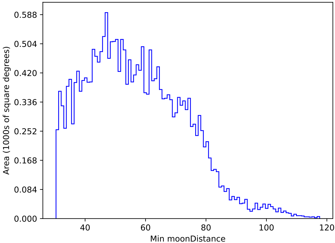
too_ignore_5_1v3.4_10yrs All sky u band: Min moonDistance
