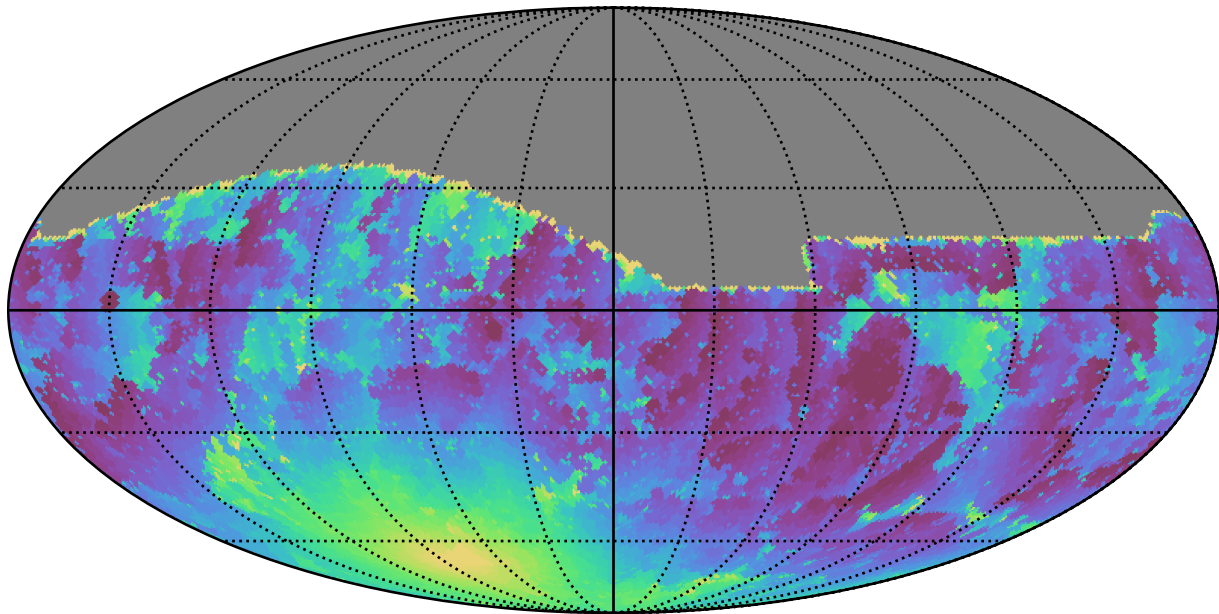
too_ignore_5_1v3.4_10yrs All sky g band: Min moonDistance
