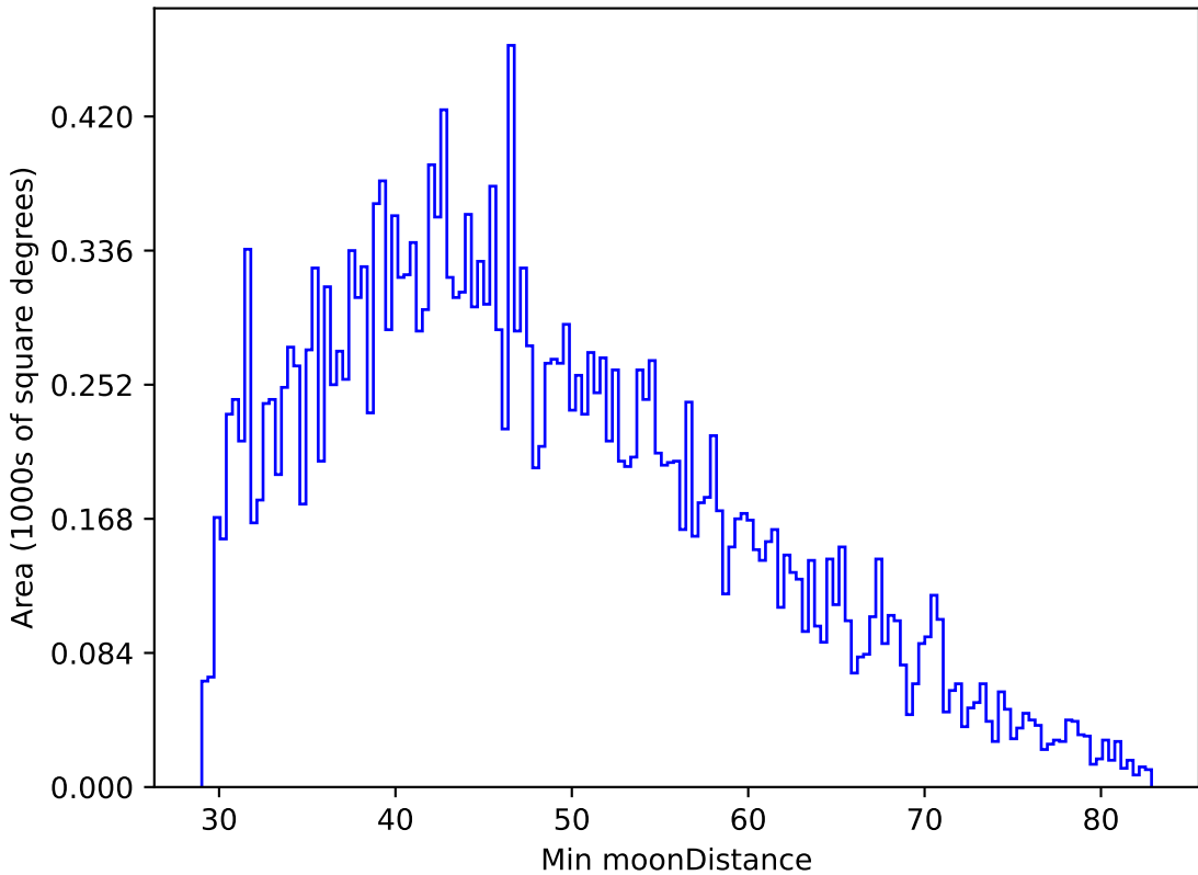
too_ignore_5_1v3.4_10yrs All sky g band: Min moonDistance
