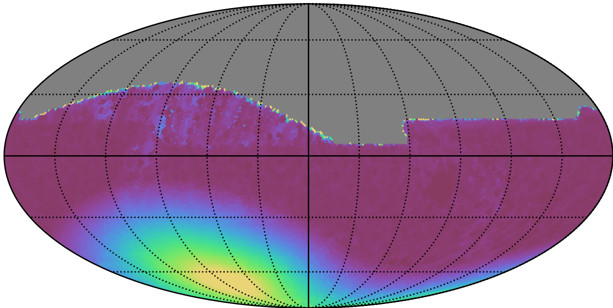
too_ignore_5_1v3.4_10yrs All sky all bands: Min moonDistance
