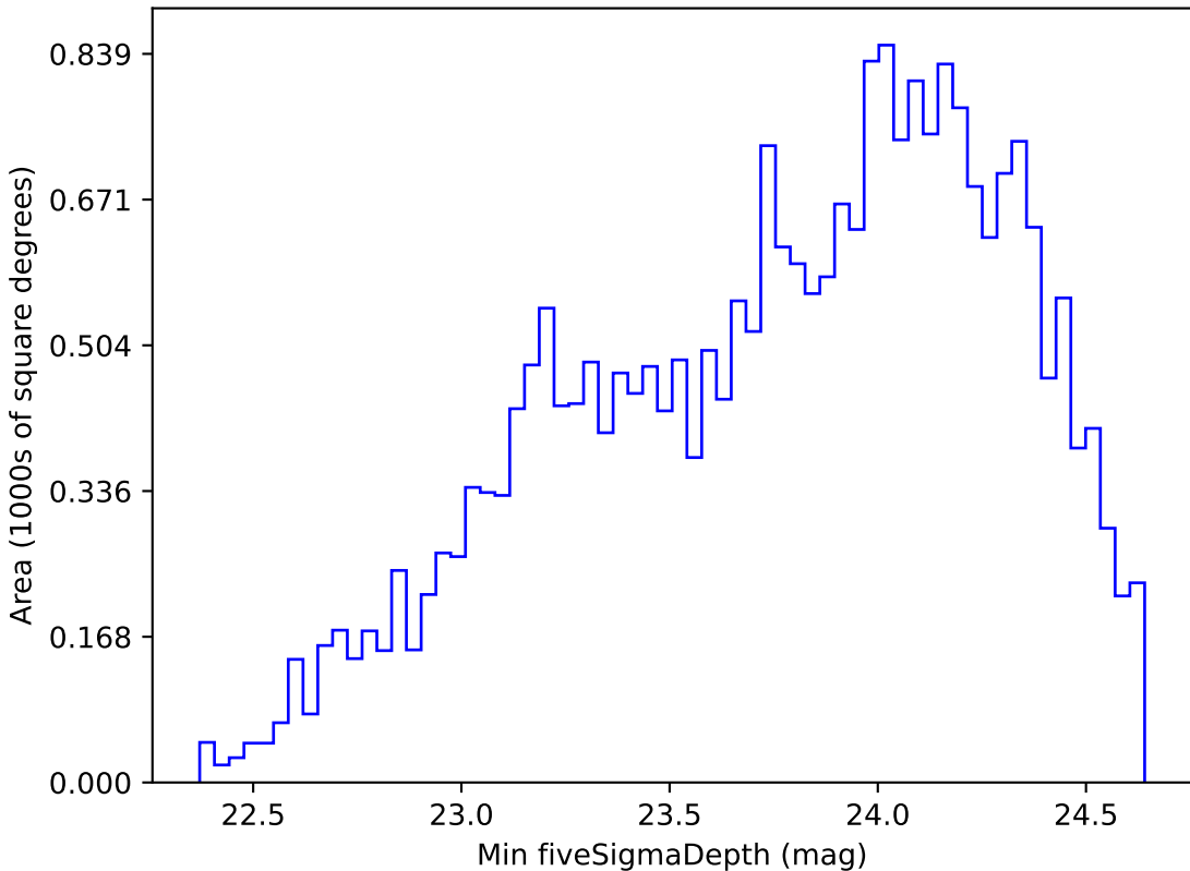
too_ignore_5_1v3.4_10yrs Yr 1 g band: Min fiveSigmaDepth
