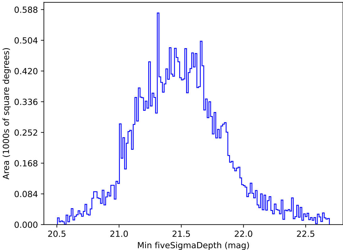
too_ignore_5_1v3.4_10yrs Yr 1 all bands: Min fiveSigmaDepth
