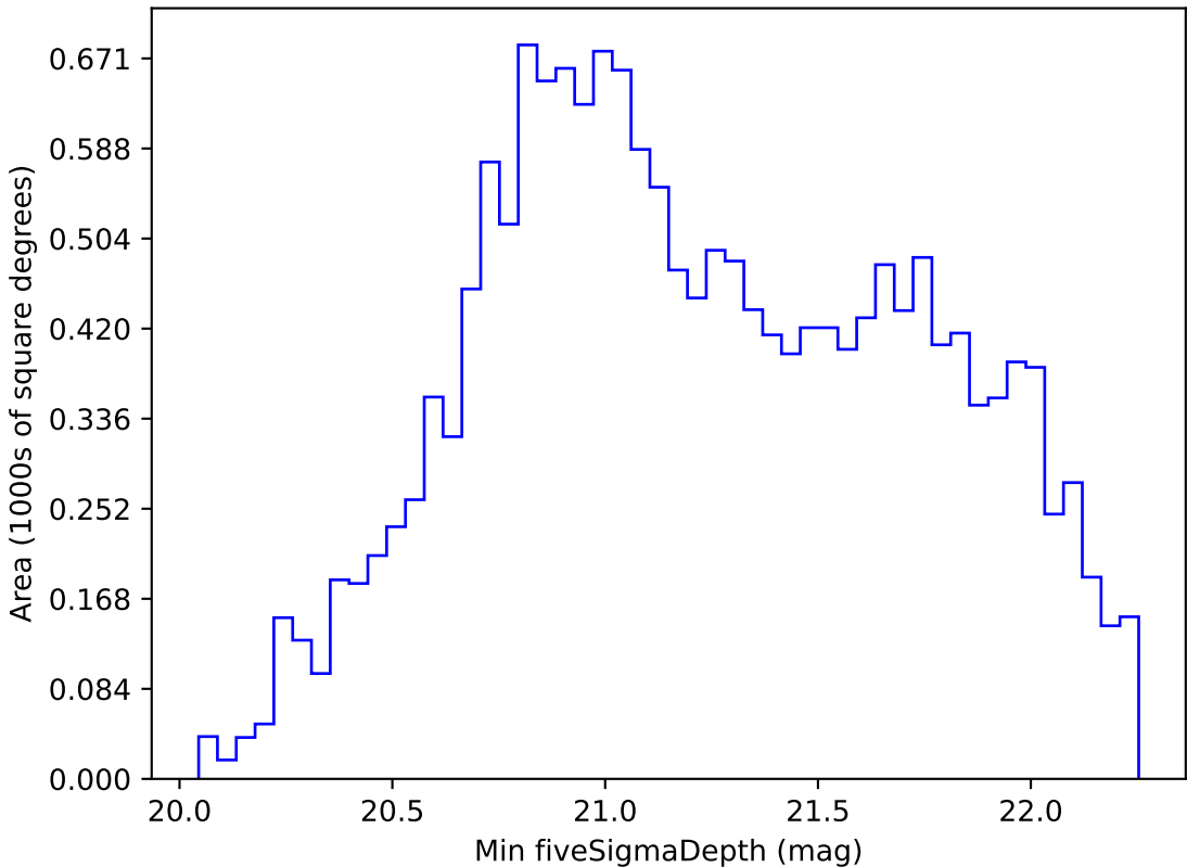
too_ignore_5_1v3.4_10yrs WFD z band: Min fiveSigmaDepth
