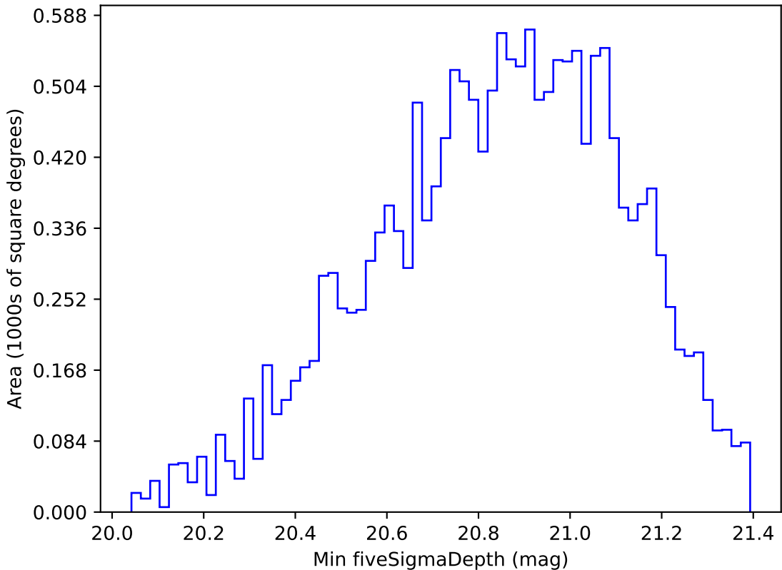
too_ignore_5_1v3.4_10yrs WFD y band: Min fiveSigmaDepth
