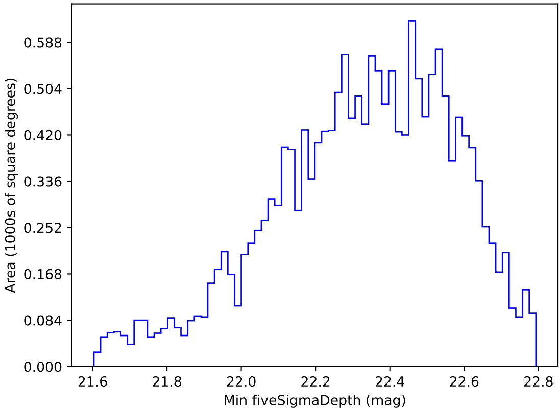
too_ignore_5_1v3.4_10yrs WFD u band: Min fiveSigmaDepth
