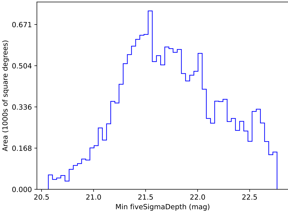
too_ignore_5_1v3.4_10yrs WFD i band: Min fiveSigmaDepth
