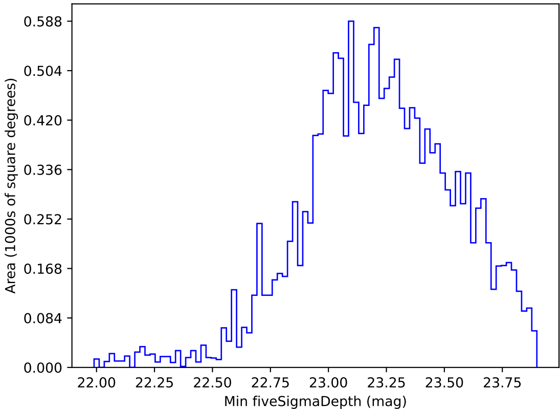
too_ignore_5_1v3.4_10yrs WFD g band: Min fiveSigmaDepth
