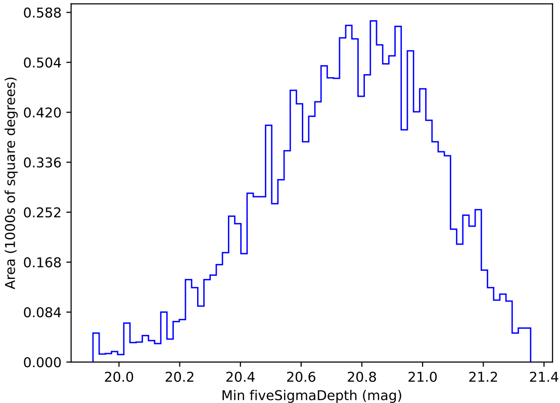
too_ignore_5_1v3.4_10yrs WFD all bands: Min fiveSigmaDepth
