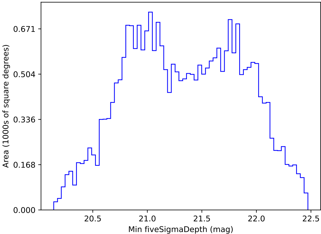
too_ignore_5_1v3.4_10yrs All sky z band: Min fiveSigmaDepth
