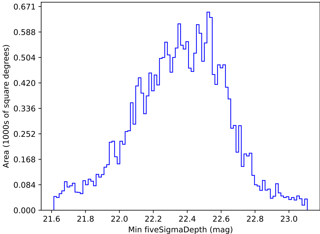
too_ignore_5_1v3.4_10yrs All sky u band: Min fiveSigmaDepth
