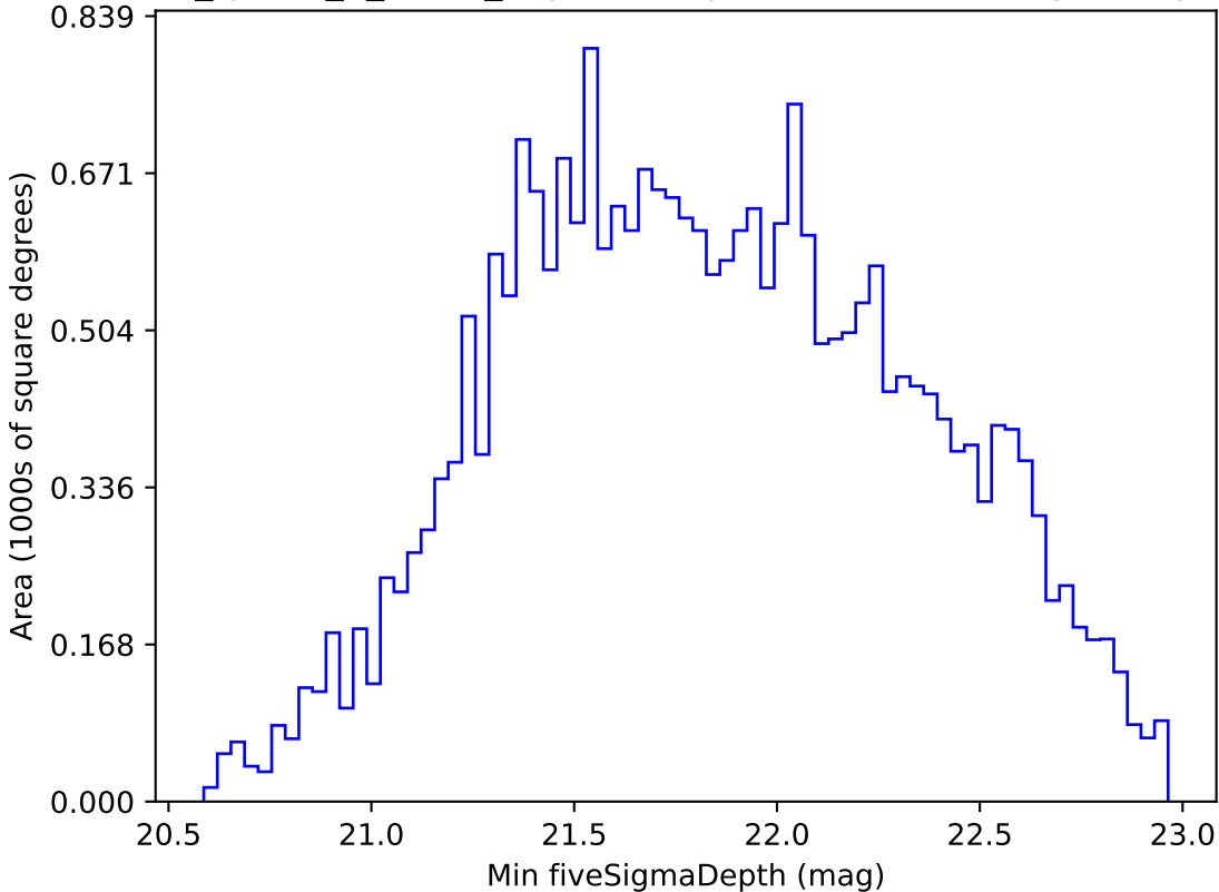
too_ignore_5_1v3.4_10yrs All sky i band: Min fiveSigmaDepth
