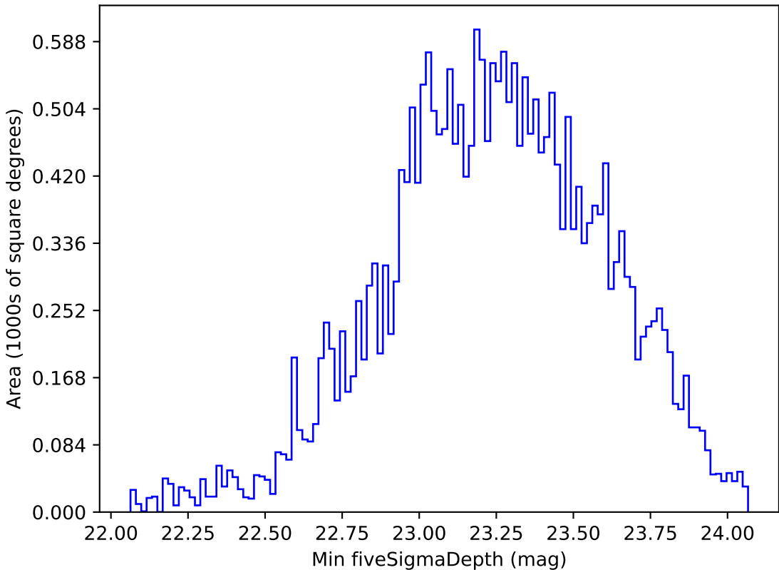
too_ignore_5_1v3.4_10yrs All sky g band: Min fiveSigmaDepth
