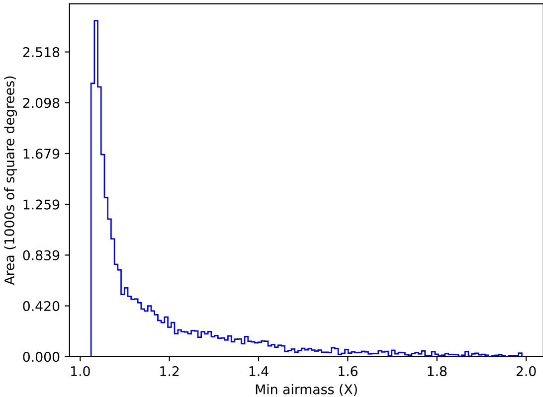
too_ignore_5_1v3.4_10yrs Yr 1 z band: Min airmass
