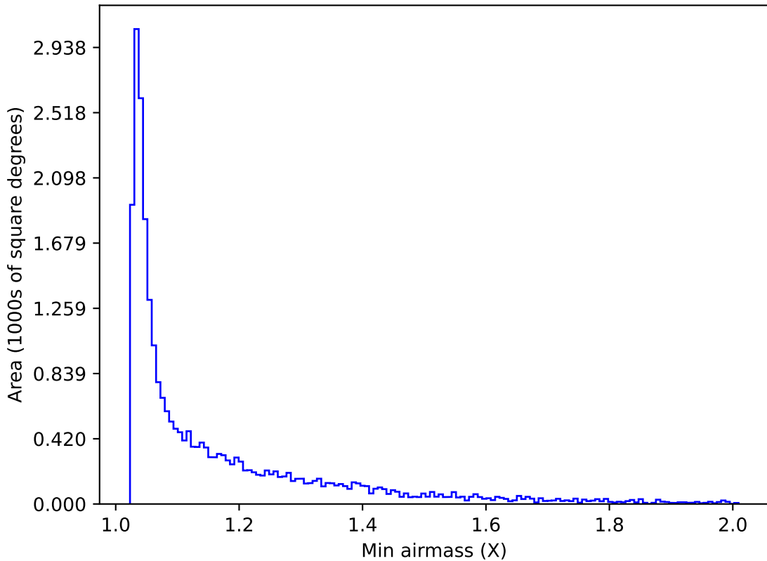
too_ignore_5_1v3.4_10yrs Yr 1 r band: Min airmass
