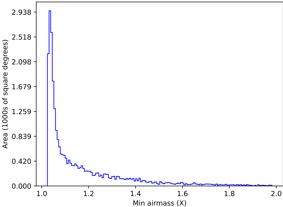
too_ignore_5_1v3.4_10yrs Yr 1 i band: Min airmass
