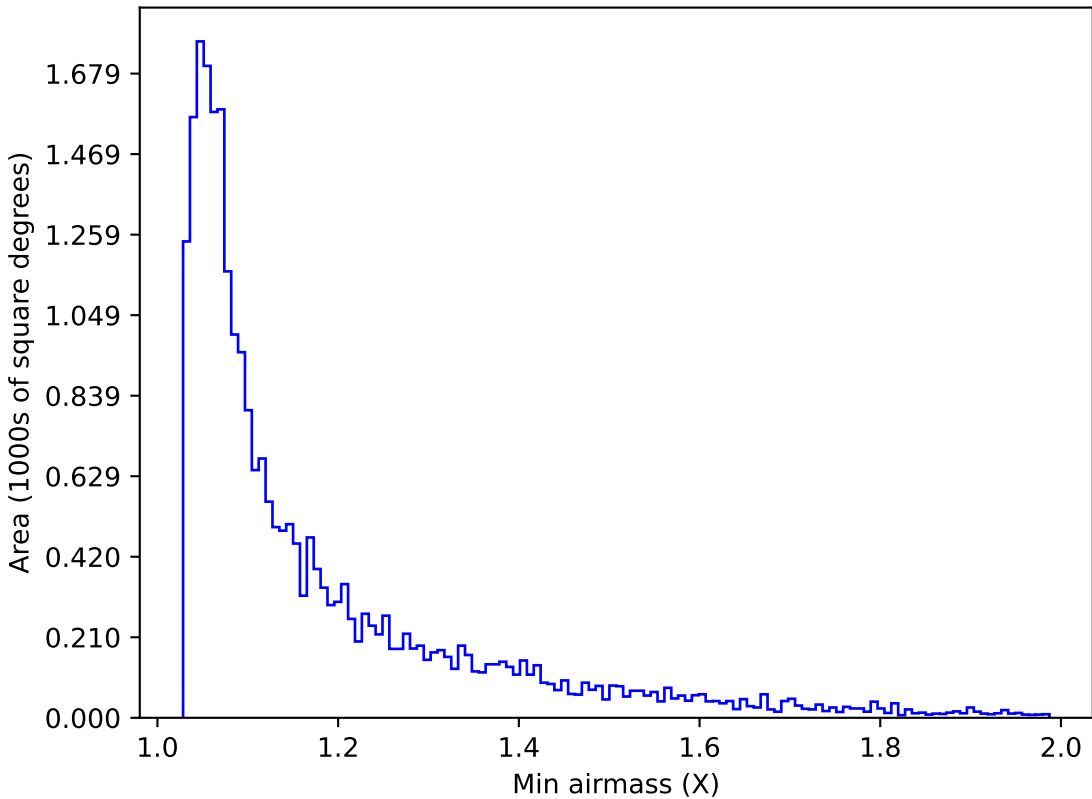
too_ignore_5_1v3.4_10yrs Yr 1 g band: Min airmass
