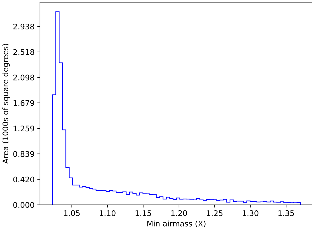
too_ignore_5_1v3.4_10yrs WFD y band: Min airmass
