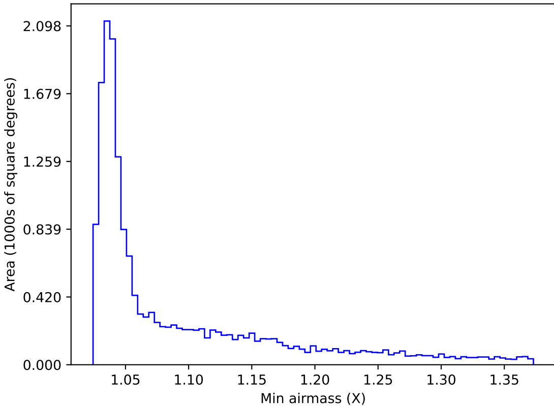
too_ignore_5_1v3.4_10yrs WFD u band: Min airmass
