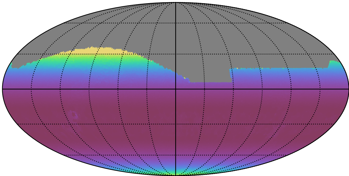
too_ignore_5_1v3.4_10yrs All sky z band: Min airmass
