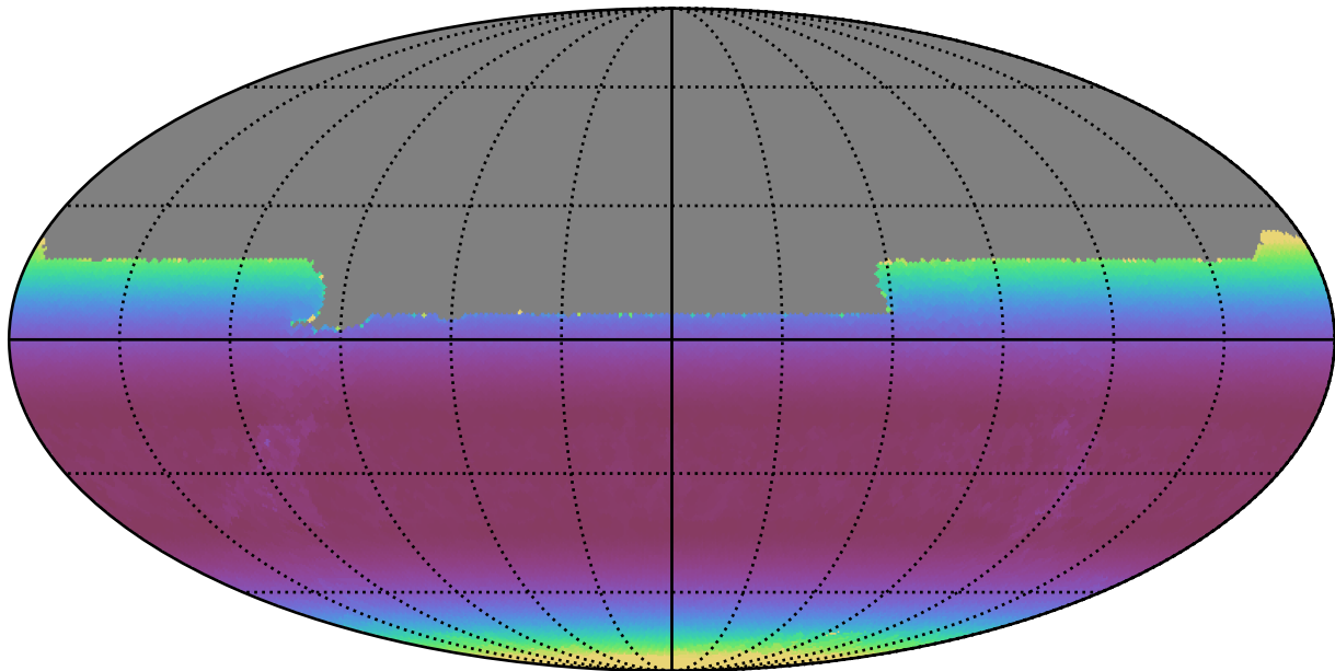
too_ignore_5_1v3.4_10yrs All sky y band: Min airmass
