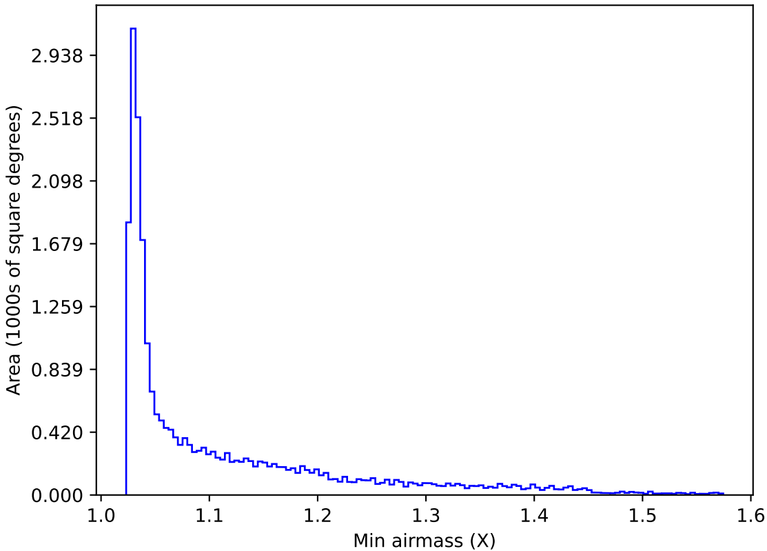
too_ignore_5_1v3.4_10yrs All sky y band: Min airmass
