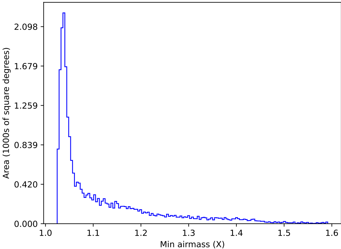
too_ignore_5_1v3.4_10yrs All sky u band: Min airmass
