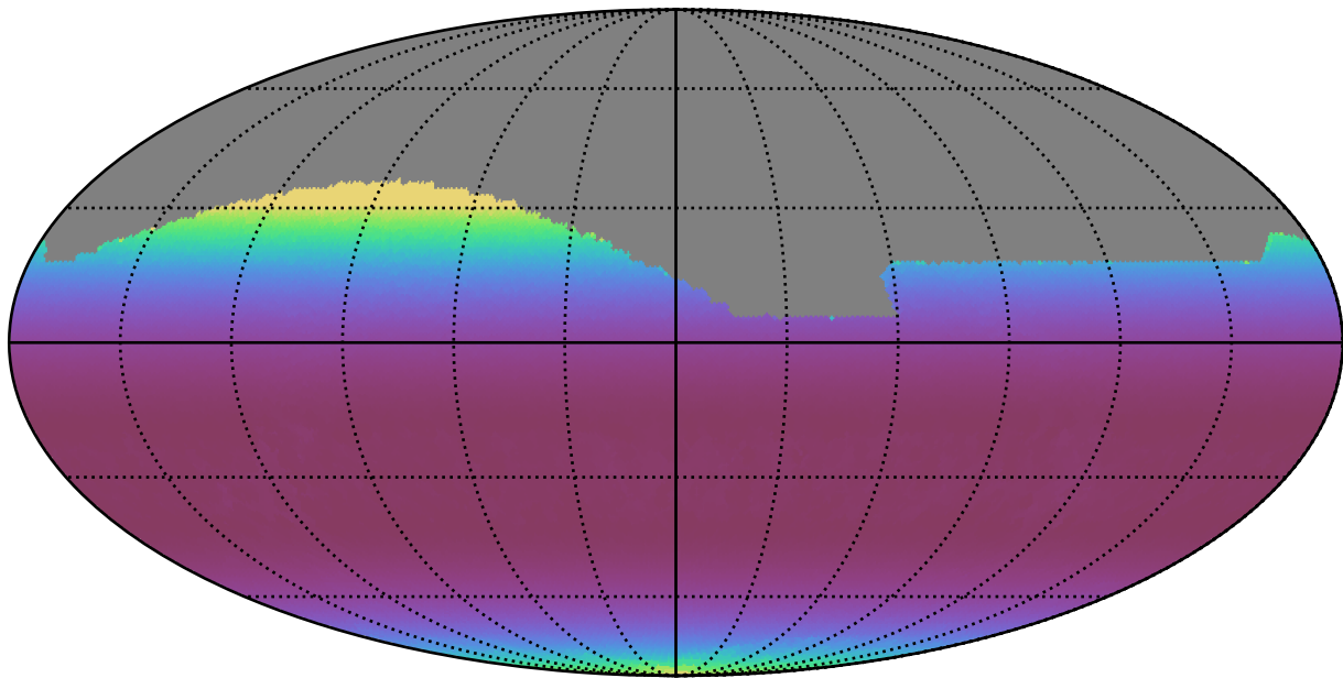
too_ignore_5_1v3.4_10yrs All sky r band: Min airmass
