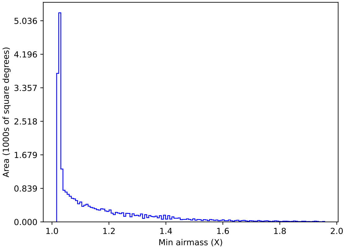
too_ignore_5_1v3.4_10yrs All sky all bands: Min airmass
