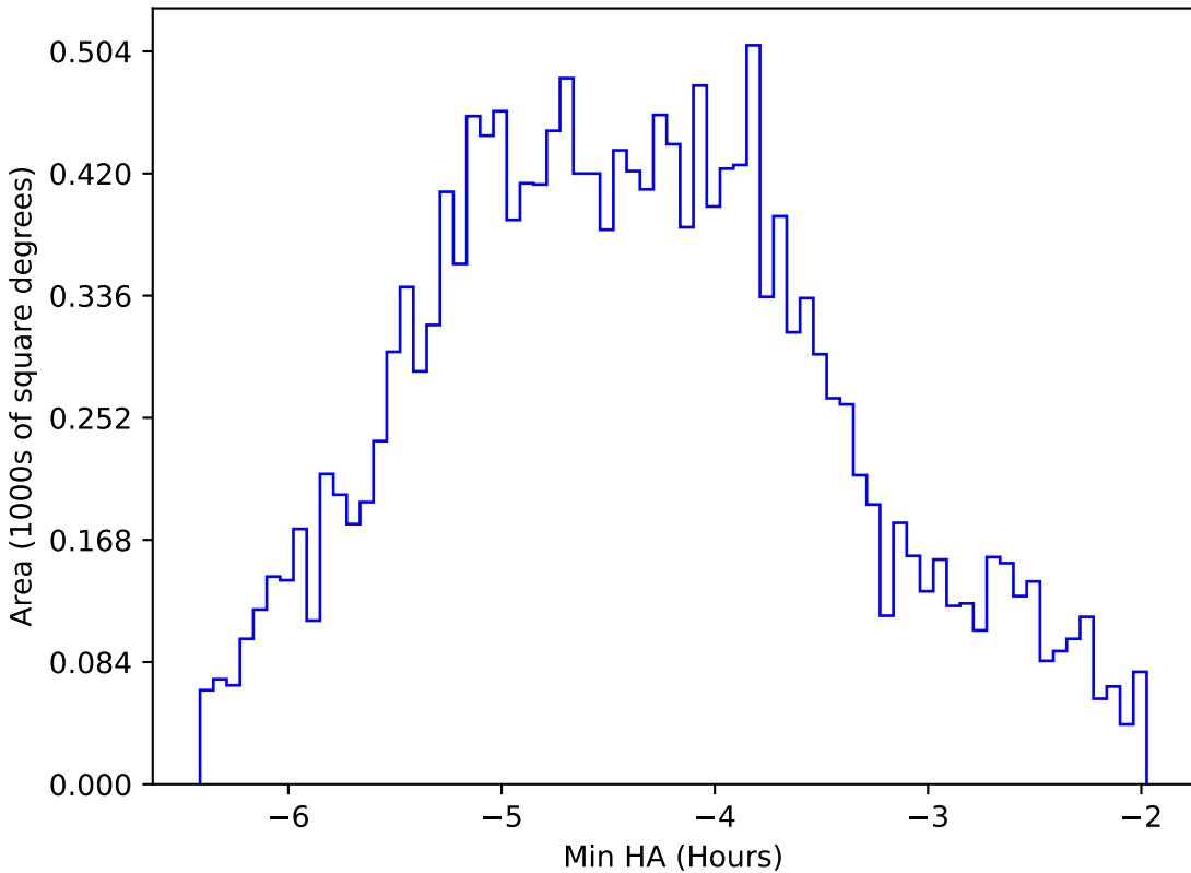
too_ignore_5_1v3.4_10yrs WFD z band: Min HA
