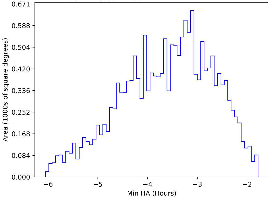
too_ignore_5_1v3.4_10yrs WFD y band: Min HA
