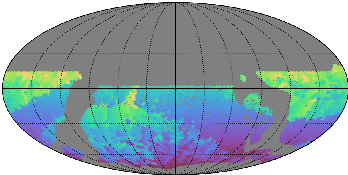
too_ignore_5_1v3.4_10yrs WFD r band: Min HA
