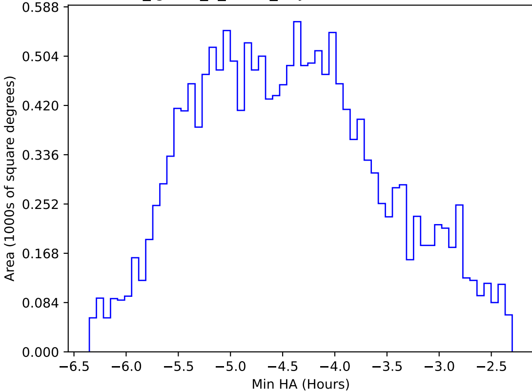
too_ignore_5_1v3.4_10yrs WFD r band: Min HA
