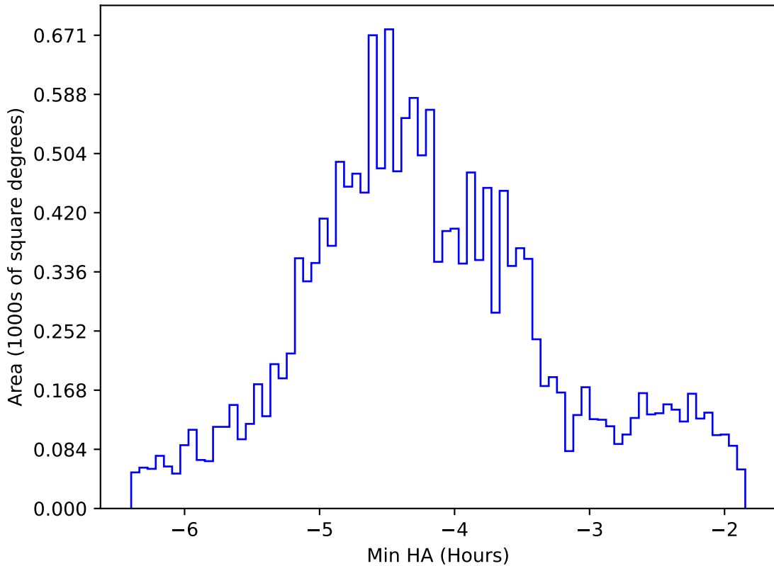
too_ignore_5_1v3.4_10yrs WFD g band: Min HA
