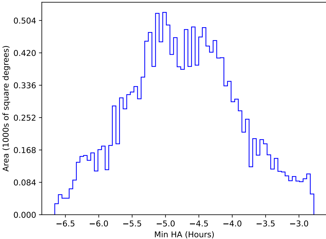
too_ignore_5_1v3.4_10yrs WFD all bands: Min HA
