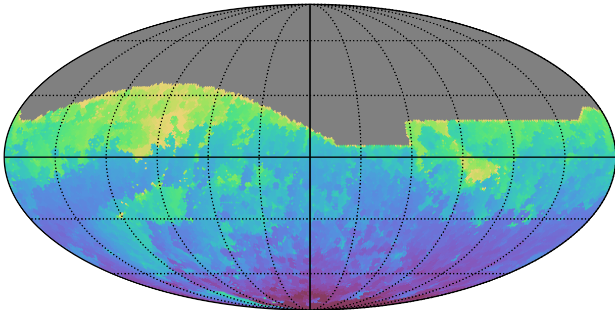
too_ignore_5_1v3.4_10yrs All sky z band: Min HA
