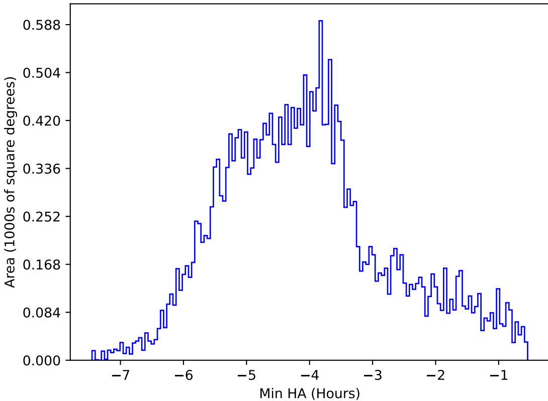
too_ignore_5_1v3.4_10yrs All sky z band: Min HA
