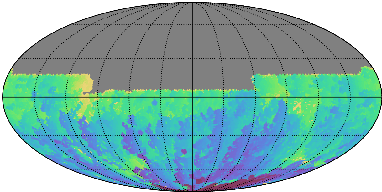
too_ignore_5_1v3.4_10yrs All sky u band: Min HA
