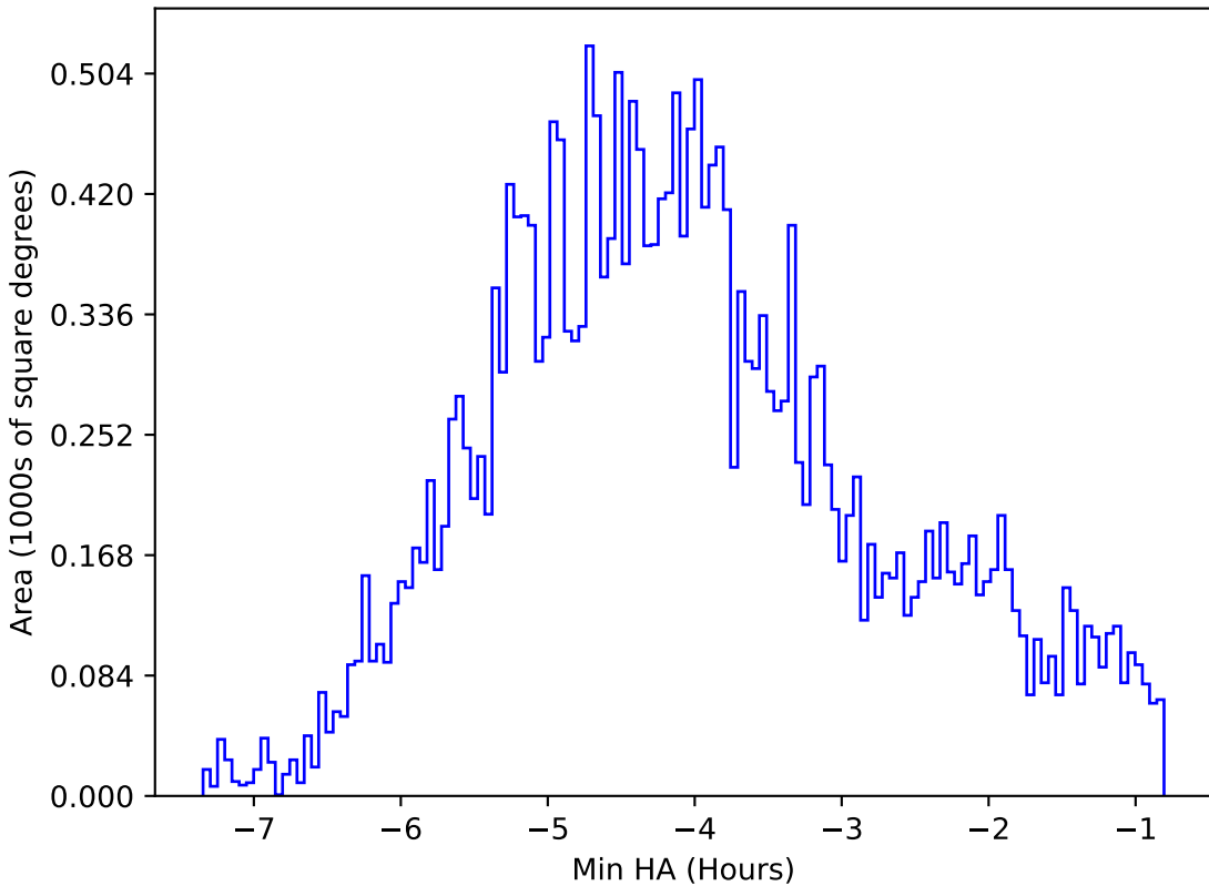
too_ignore_5_1v3.4_10yrs All sky i band: Min HA
