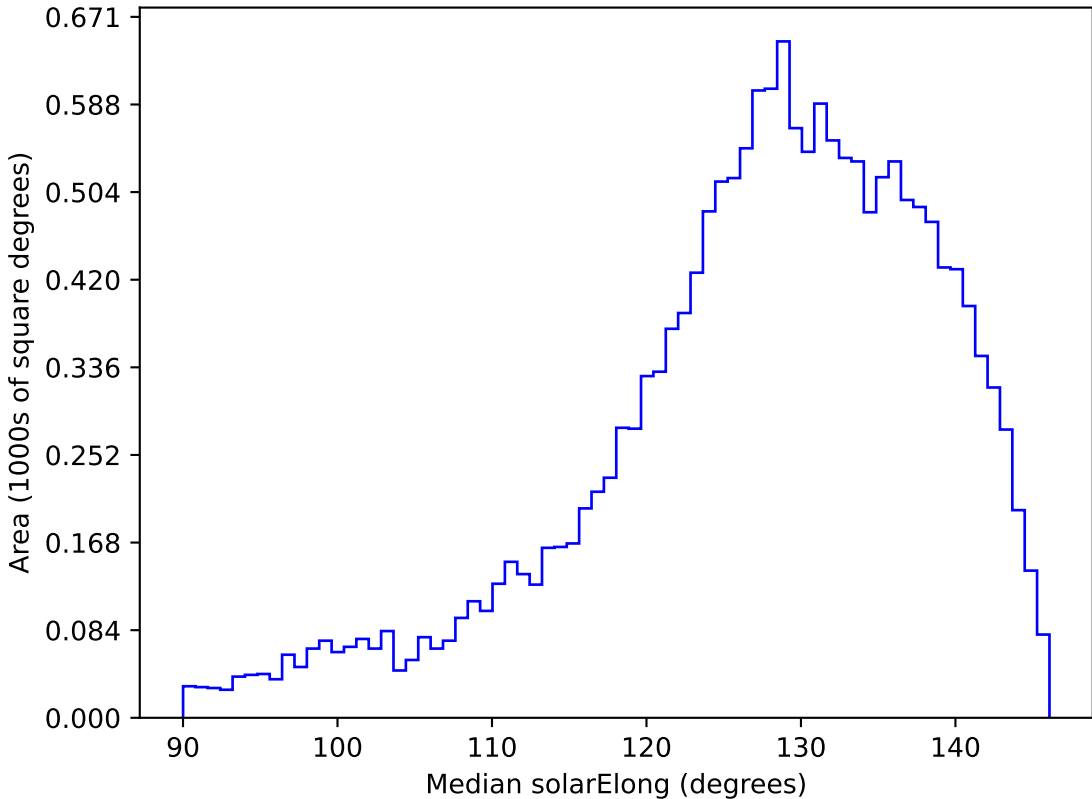
too_ignore_5_1v3.4_10yrs WFD z band: Median solarElong
