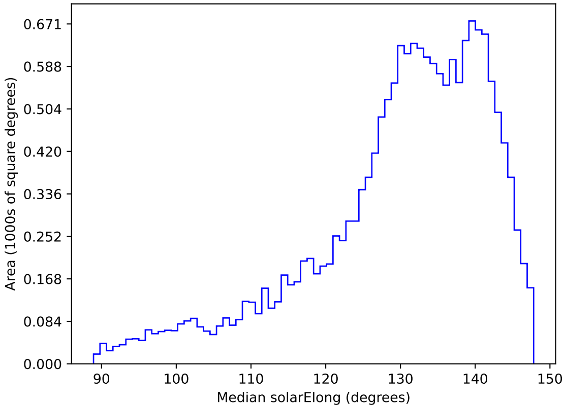
too_ignore_5_1v3.4_10yrs WFD y band: Median solarElong
