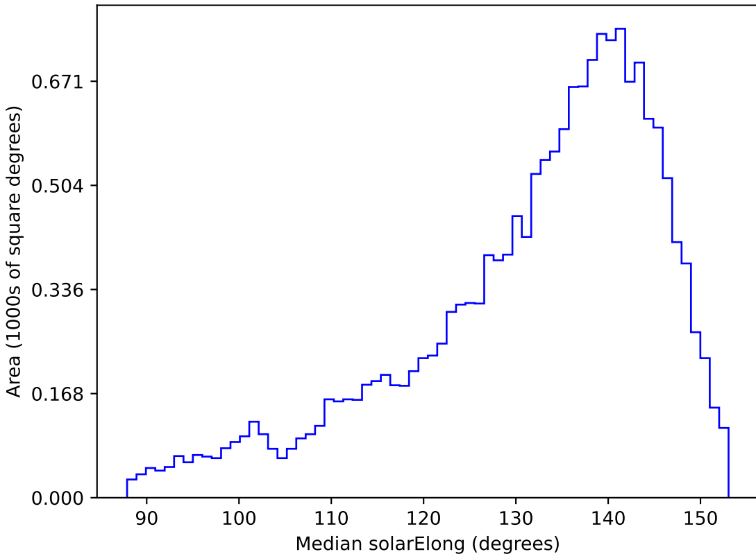
too_ignore_5_1v3.4_10yrs WFD u band: Median solarElong
