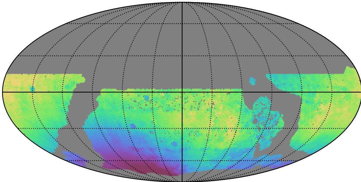
too_ignore_5_1v3.4_10yrs WFD g band: Median solarElong
