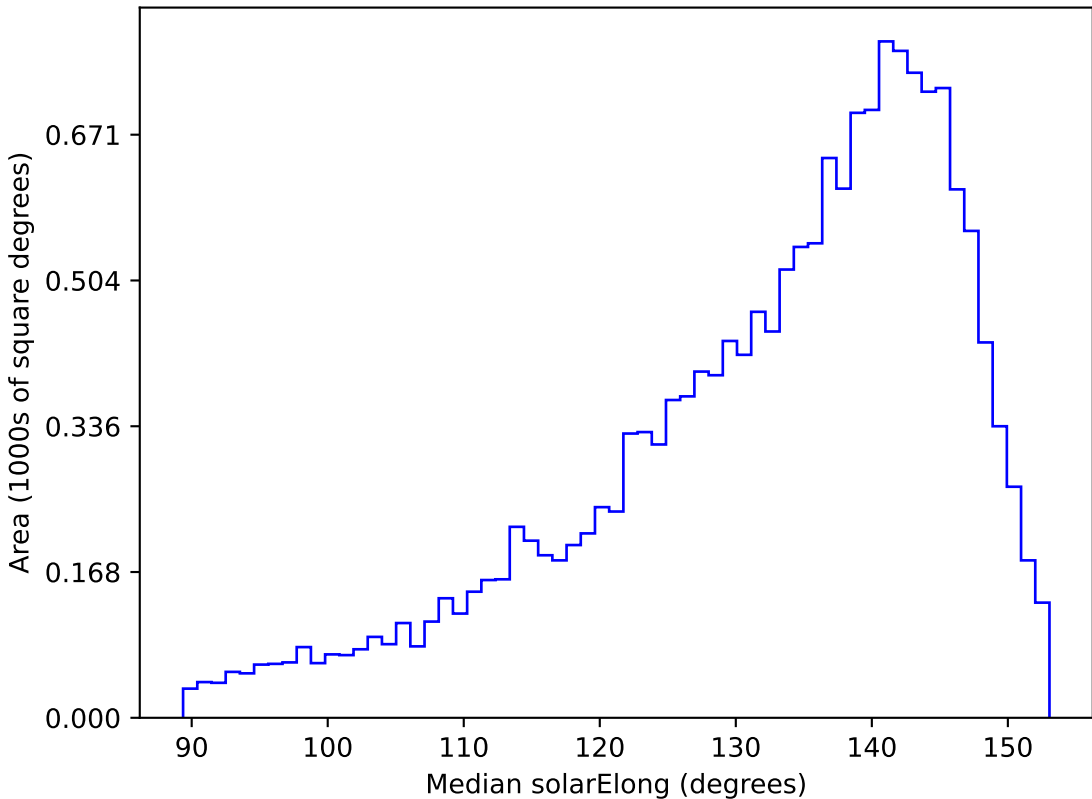
too_ignore_5_1v3.4_10yrs WFD g band: Median solarElong
