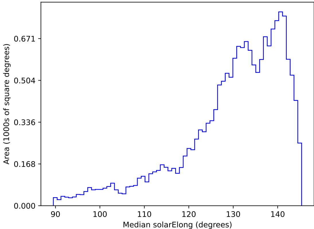
too_ignore_5_1v3.4_10yrs WFD all bands: Median solarElong
