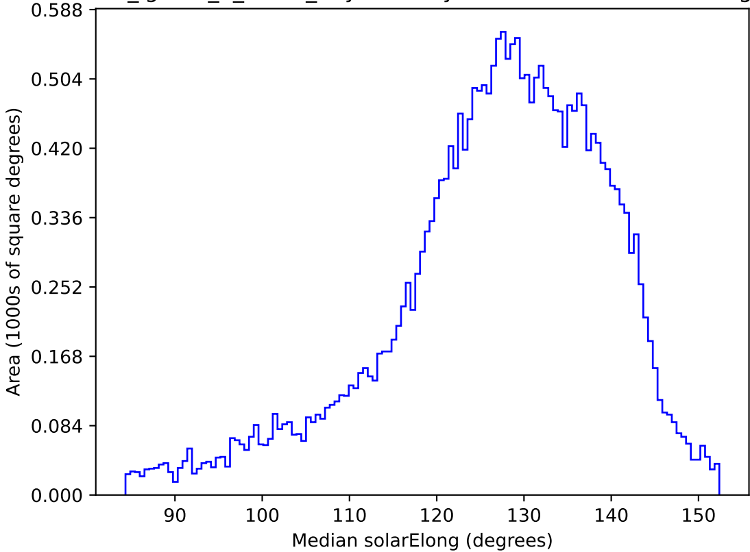
too_ignore_5_1v3.4_10yrs All sky z band: Median solarElong
