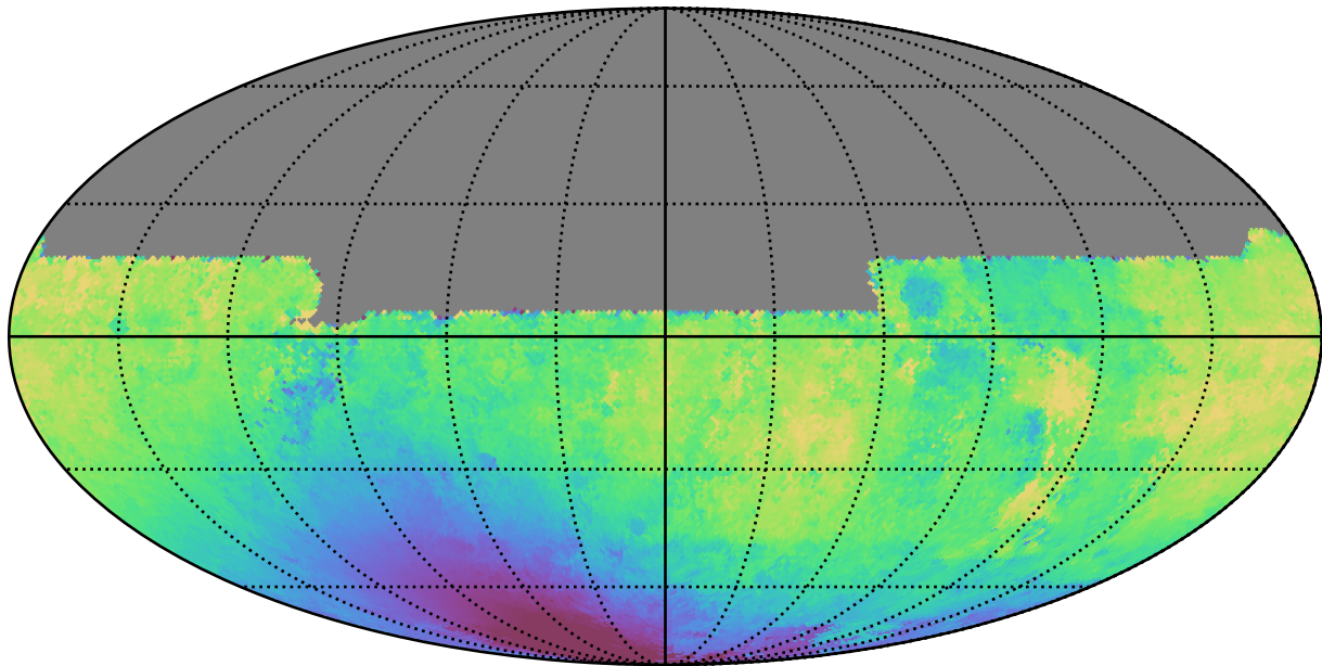
too_ignore_5_1v3.4_10yrs All sky y band: Median solarElong
