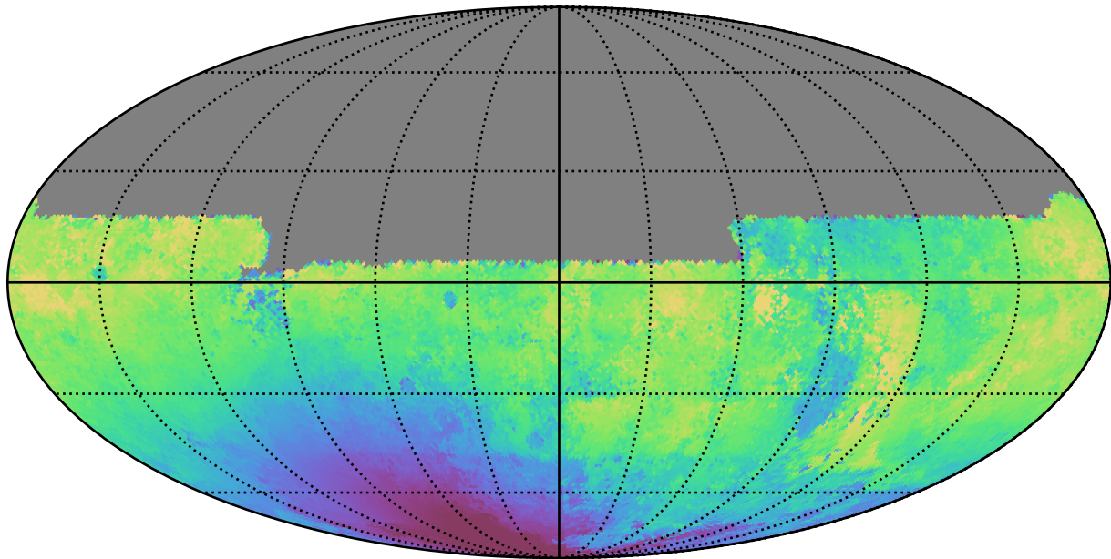
too_ignore_5_1v3.4_10yrs All sky u band: Median solarElong
